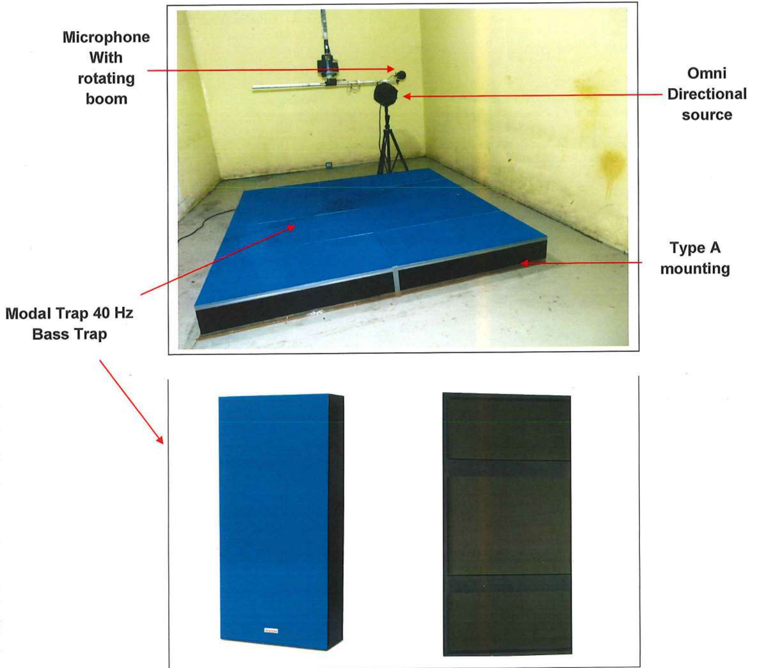
Figure 1: Test set up for mounting and testing of Modal Trap 40 Hz Bass Trap with Type A mounting in reverberation chamber
